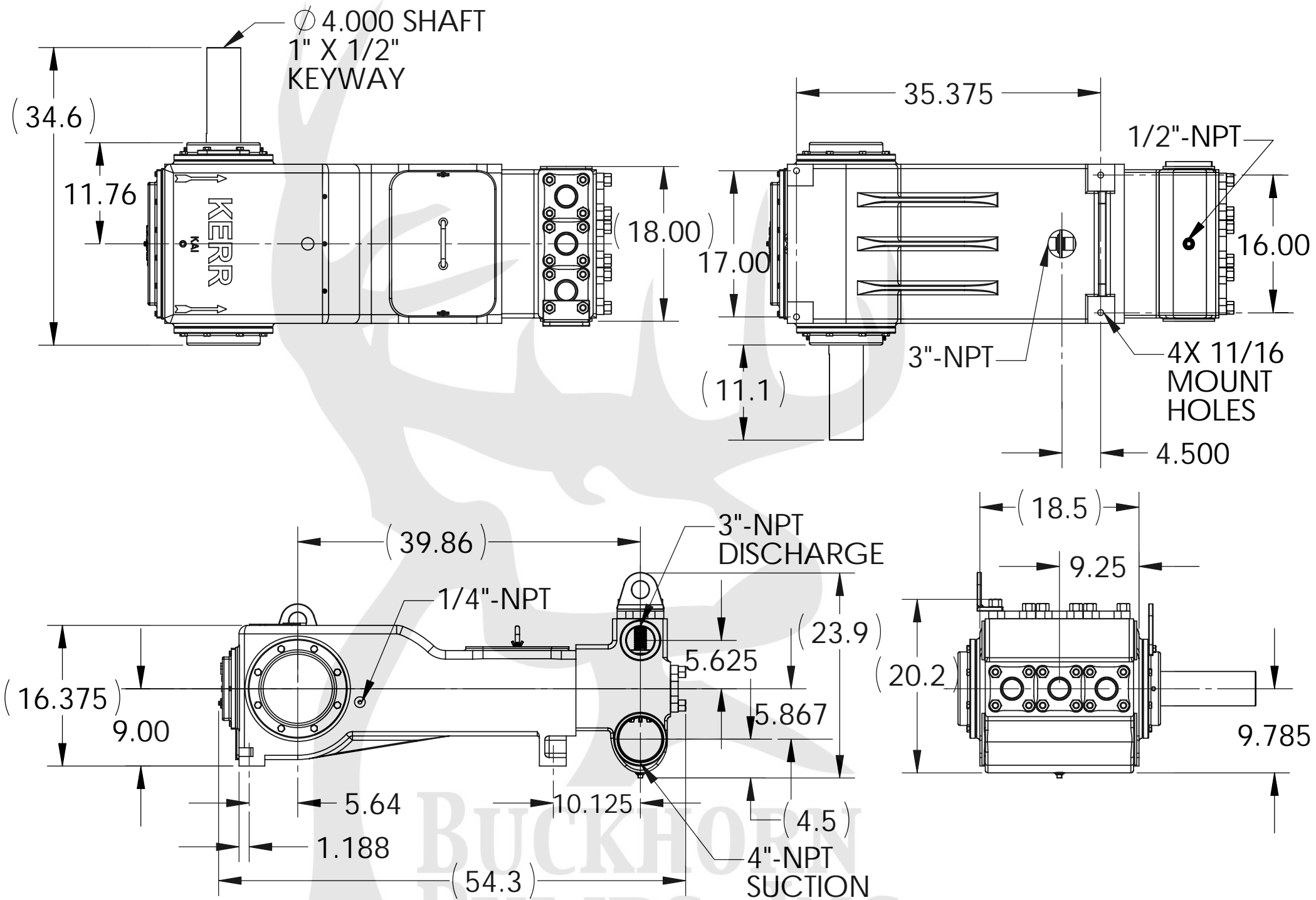
GENERAL DIMENSIONS FOR KA-3500
