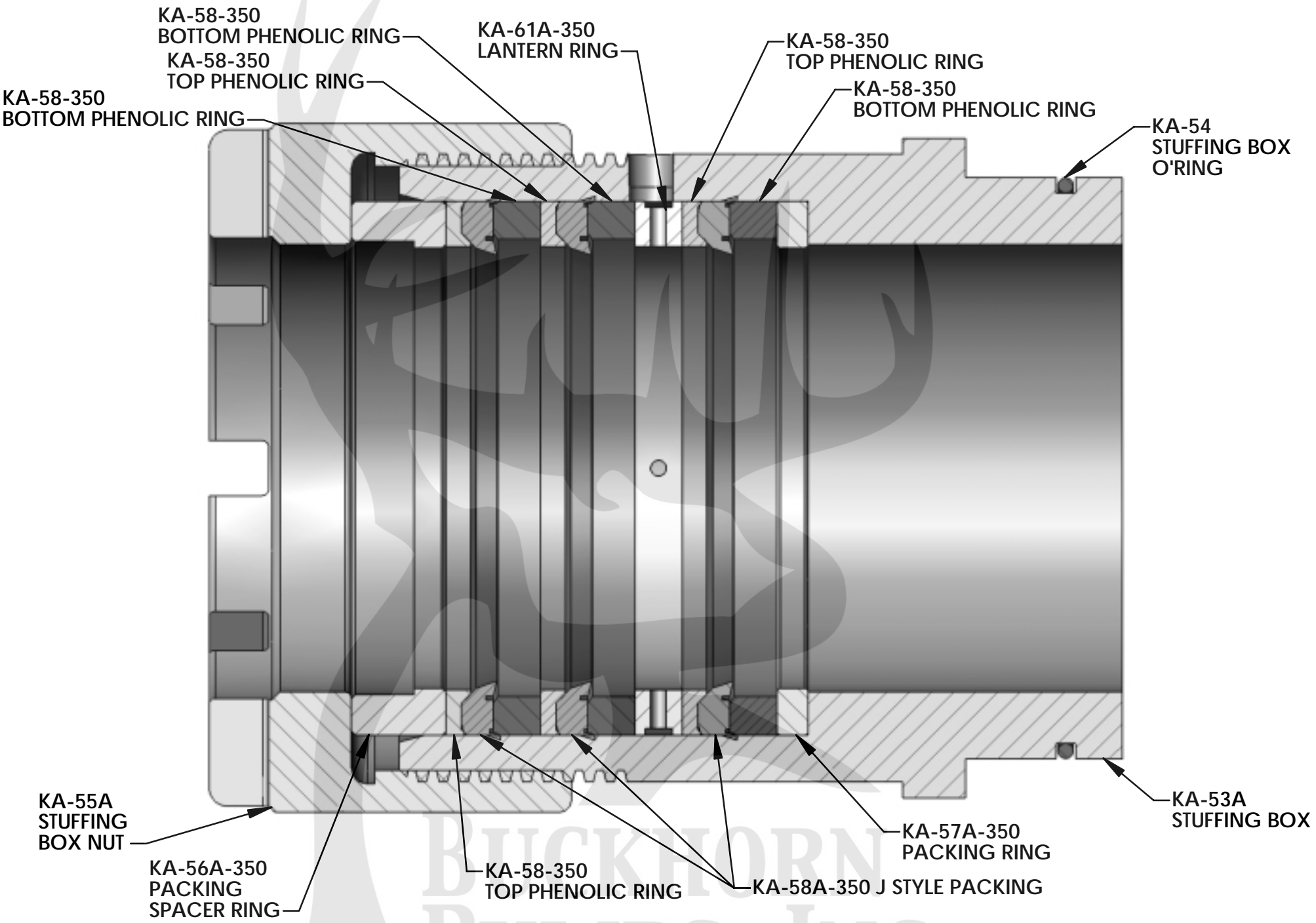
KA-3500 "A" BOX PACKING ARRANGEMENT (FOR 3.500" PLUNGERS)
