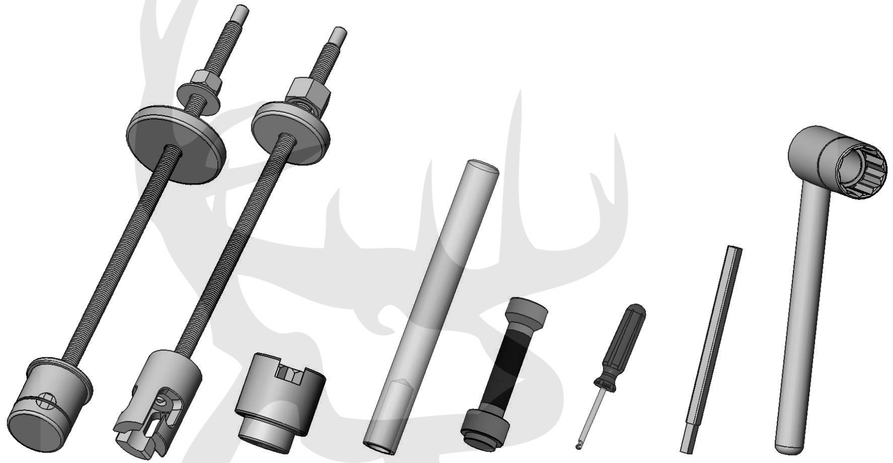
KA-68M WING- GUIDED SEAT TRI-PIN TYPE PULLER ASS'Y
