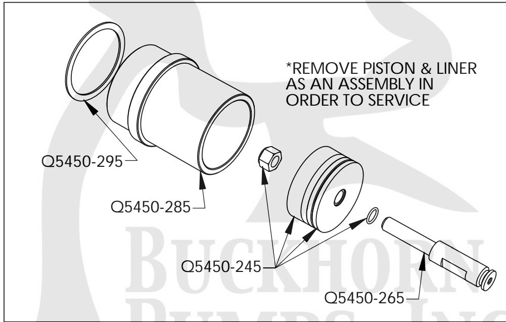
Q5450PT PARTS ILLUSTRATION
