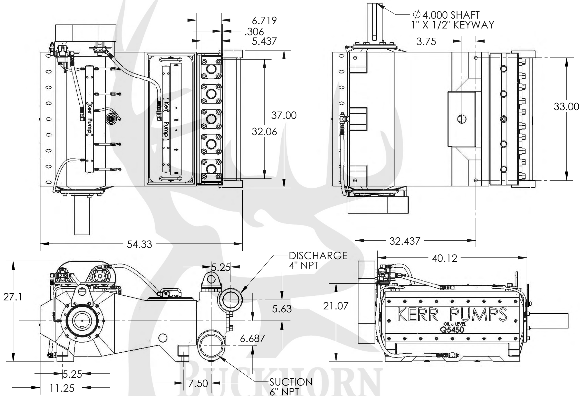
Q5450PT - RH GENERAL DIMENSIONS
