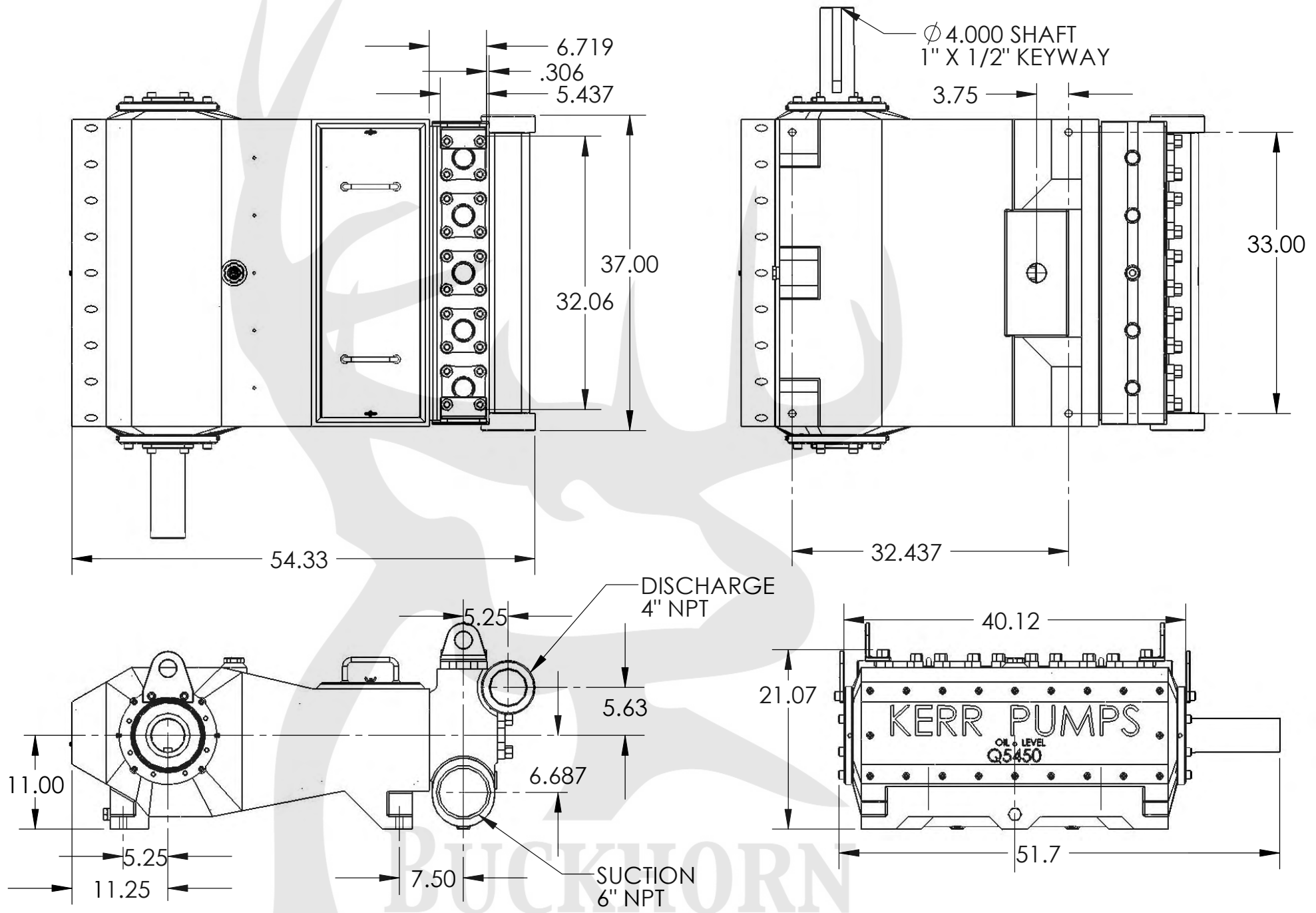
Q5450PT GENERAL DIMENSIONS
