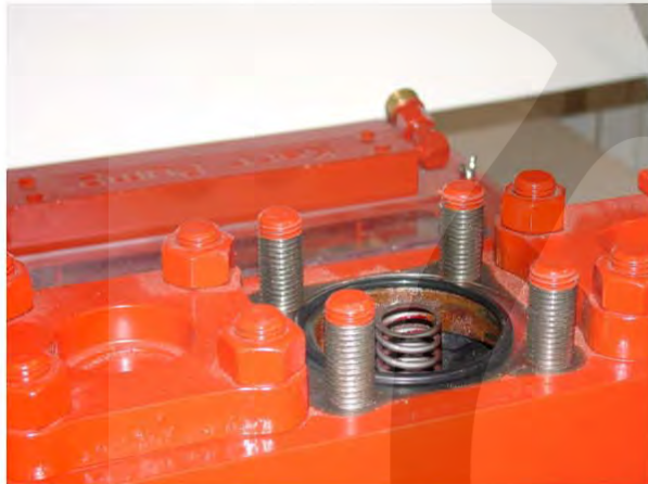
16.) Install the discharge spring.
